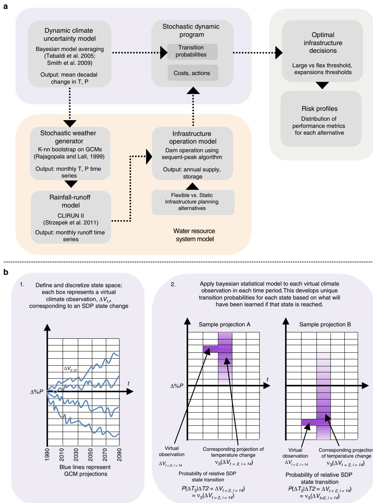
Fig. 1 Schematic of integrated modeling framework. a Full planning framework. b Detail on characterizing transition probabilities using Bayesian statistical model applied to each virtual climate observation
